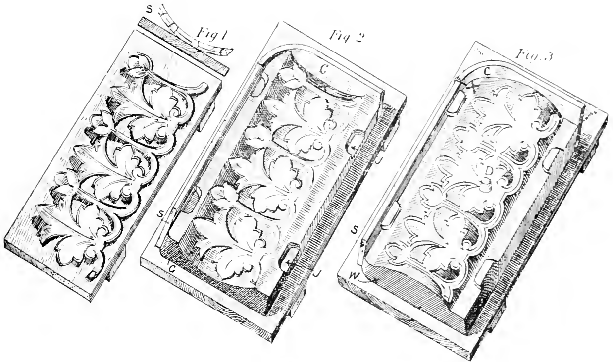
NO. 91.—MAKING A FRONT AND BACK WAX MOLD.
